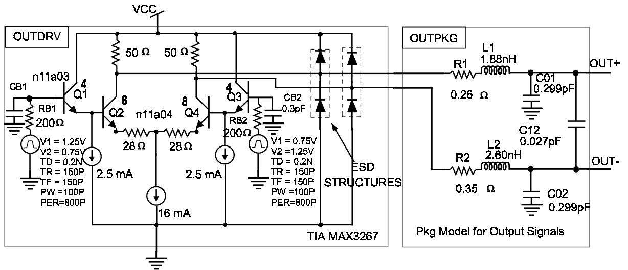
Figure 1. Output signal buffer for the MAX3267 including a simplified package model.
