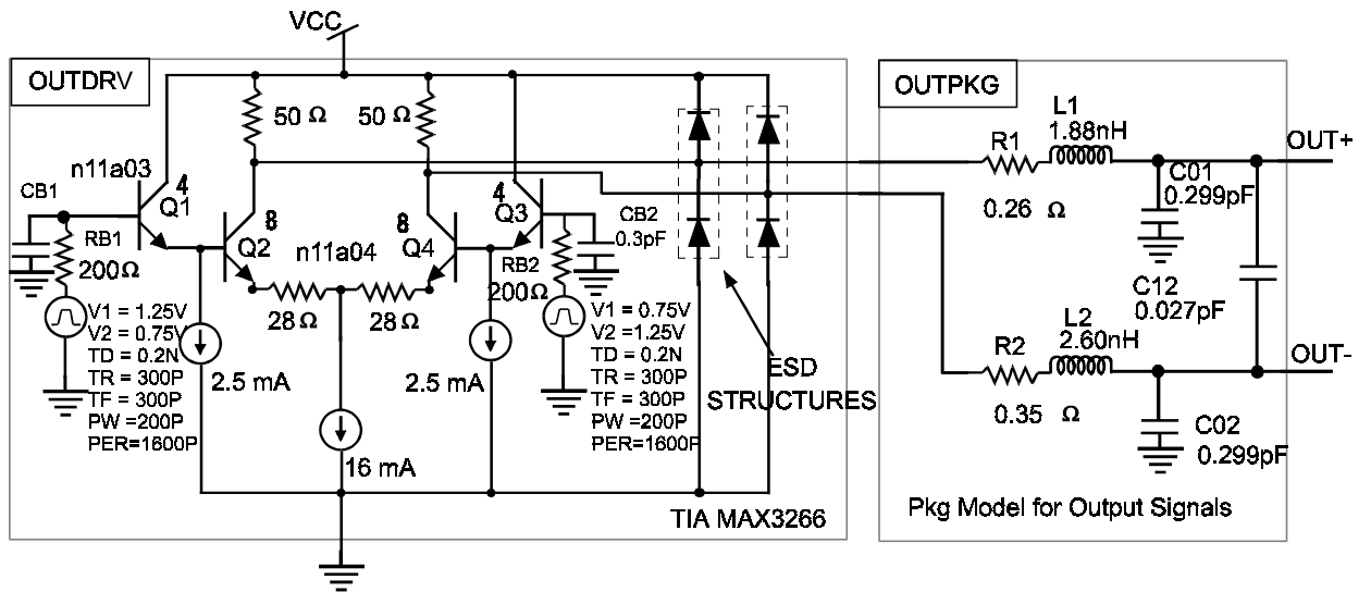
Figure 1. Output signal buffer for the MAX3266 including a simplified package model.
