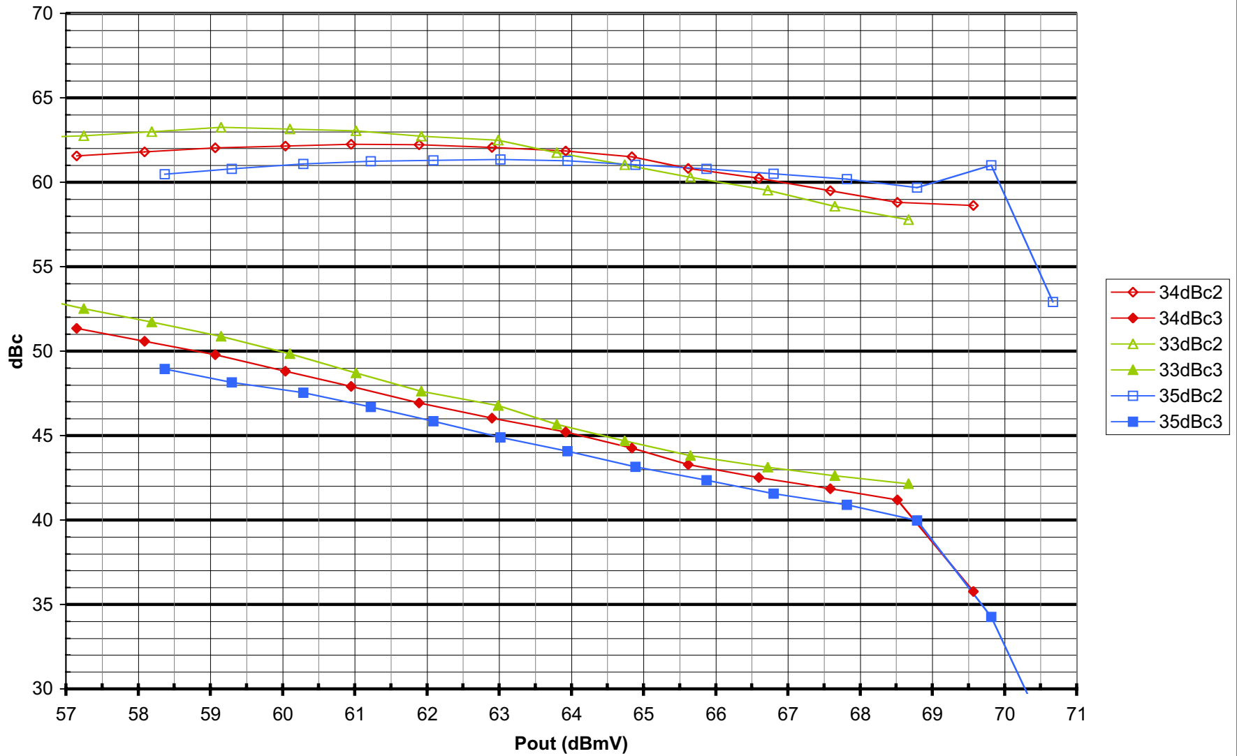
2nd 3rd Harmonics vs. Pout MAX3509 65MHz 2:1 Pin=33, 34, 35dBmV
