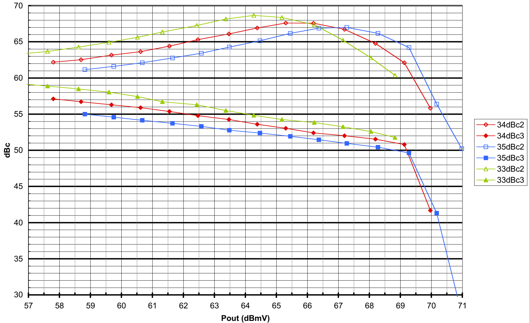
2nd 3rd Harmonic vs Pout MAX3509 22MHz 2:1 Pin=33,34,35dBmV
