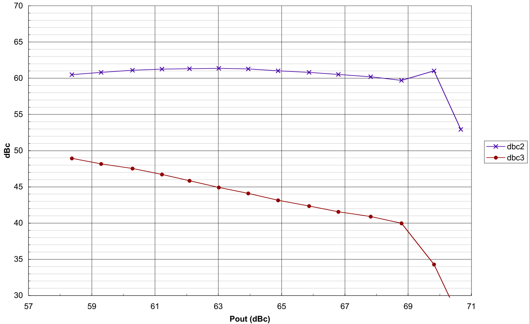
2nd 3rd Harmonic vs. Pout MAX3509 65MHz 2:1 Pin=35dBmV
