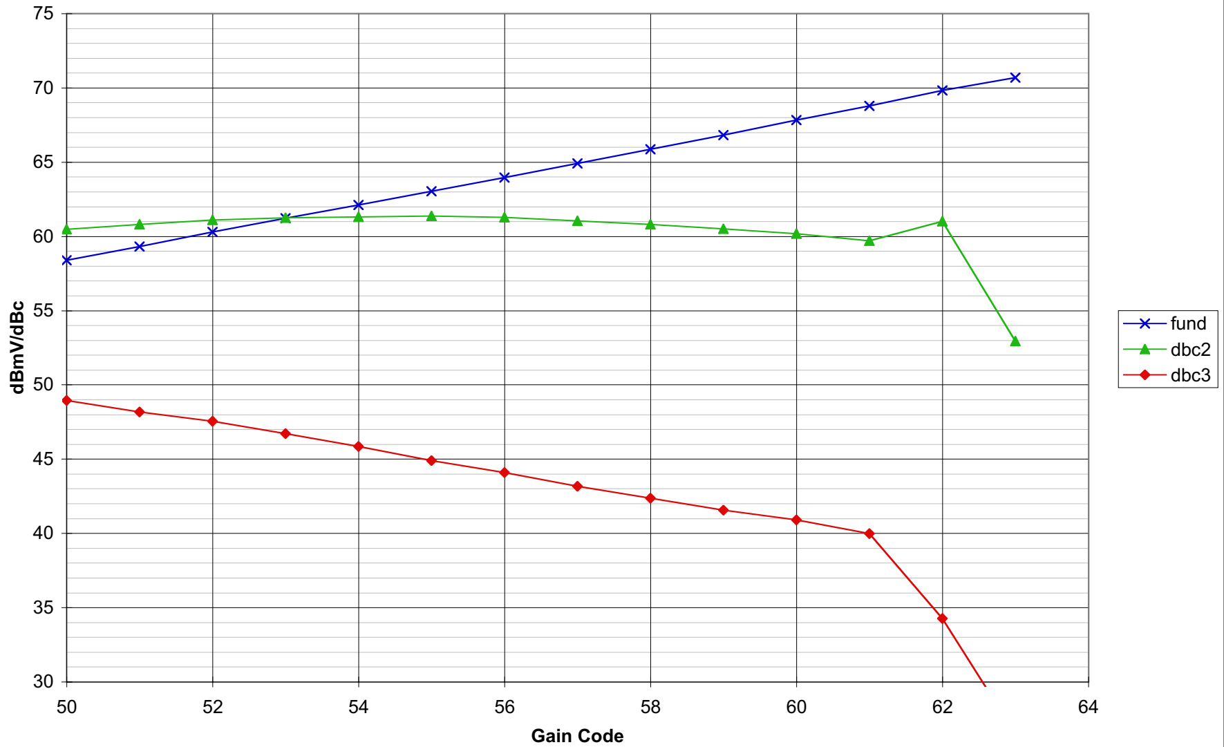
Pout, Harmonics vs Gain Code MAX3509 65MHz 2:1 Pin=35dBmV
